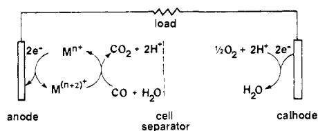
Scheme I. Generalized CO/O 2 Fuel Cell Employing the Two-Electron Redox Couple M (n+2)/n+ of a Homogeneous Electrocatalyst a
