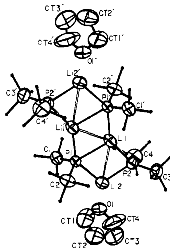
Figure 1. General view of [\text{Li}_2(\mu_3\text{-}t\text{-Bu}_2\text{P})(\mu_2\text{-}t\text{-Bu}_2\text{P})(\text{C}_4\text{H}_8\text{O})]_2 ( 1 ). For clarity methyl groups of the t -Bu units are represented as sticks.
